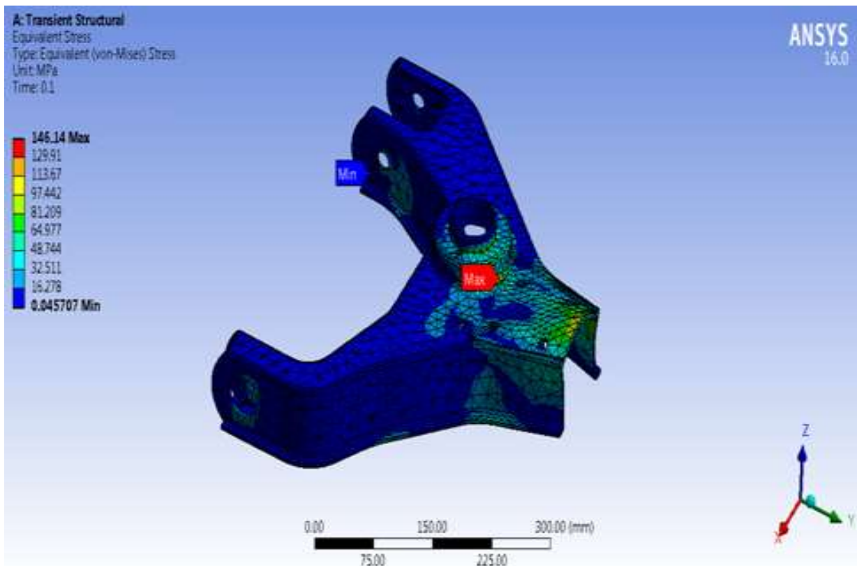
Fig 7: Von Misses Stresses on Upper Control Arm
