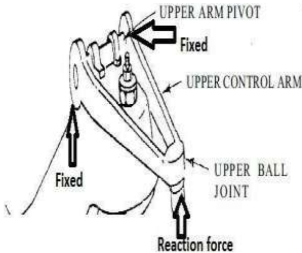
Fig 2: Boundary forces for Static Condition
