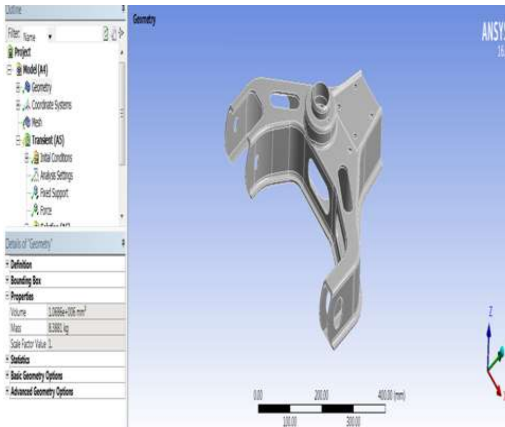
Fig 10: Upper Control Arm with Profile Modification
