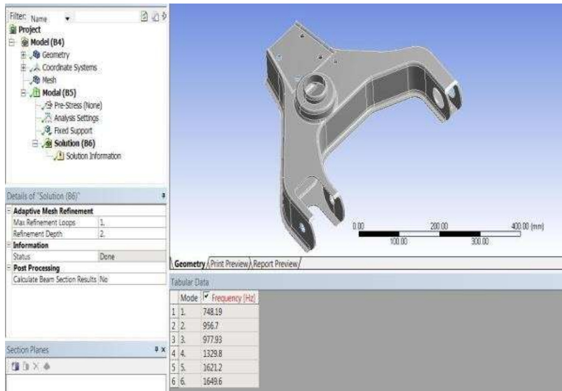
Fig 9: Natural Frequency of Upper Control Arm
