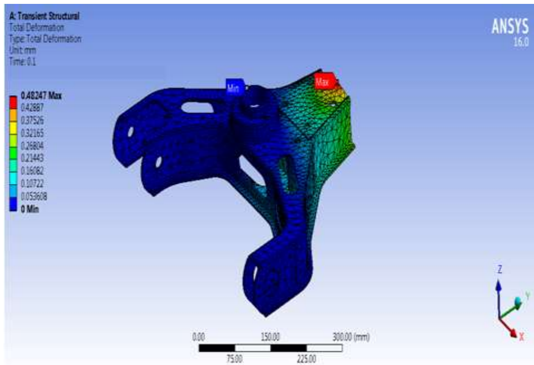
Fig 13: Deformation of Upper Control Arm
