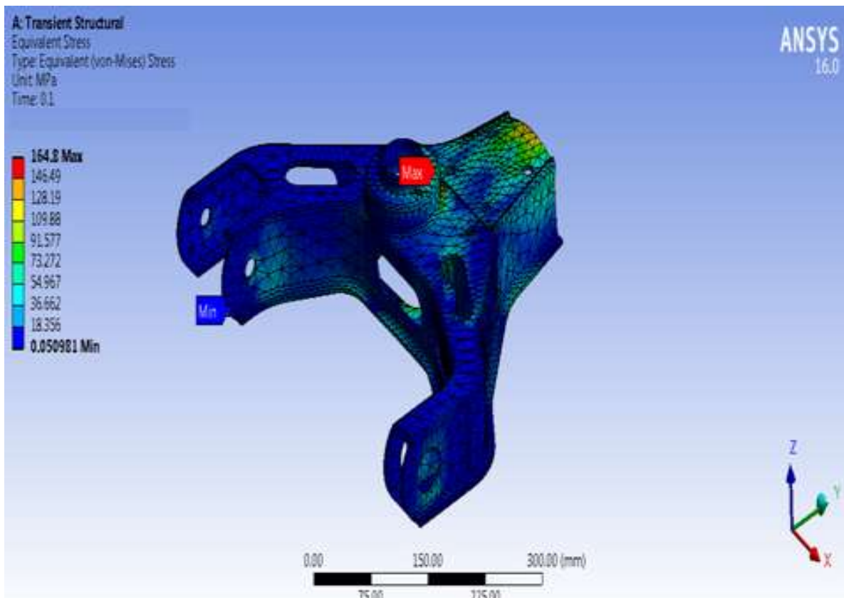
Fig 12: Von Misses Stresses on Upper Control Arm
