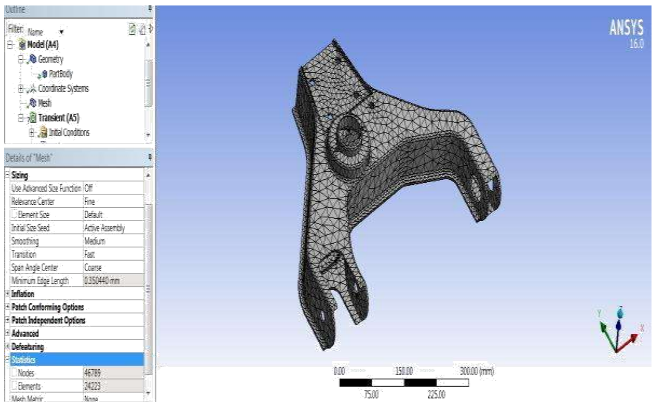
Fig 6: Meshing of Upper Control Arm using Tetrahedral Element
