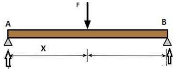
Fig 4: Force on the Axle Simply supported beam Taking moment at point A
