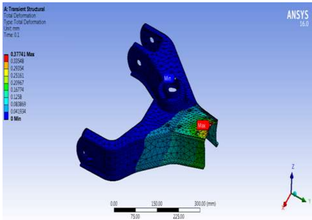
Fig 8: Deformation of Upper Control Arm
