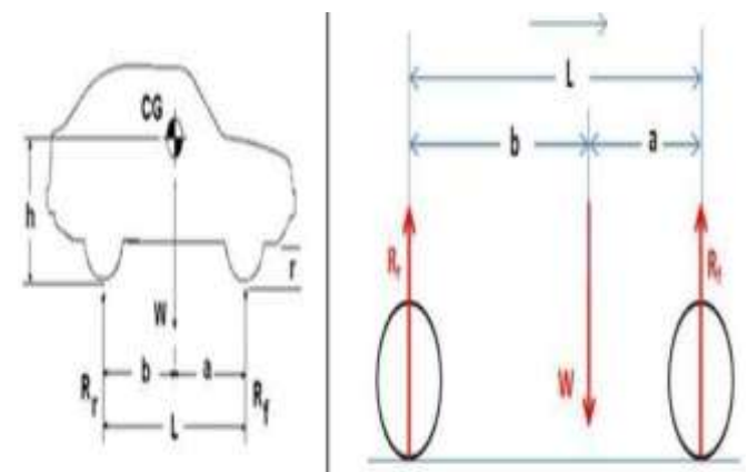
Fig 1: Forces on Stationary Car Total weight of the car = 2300 kg = 22563 N
