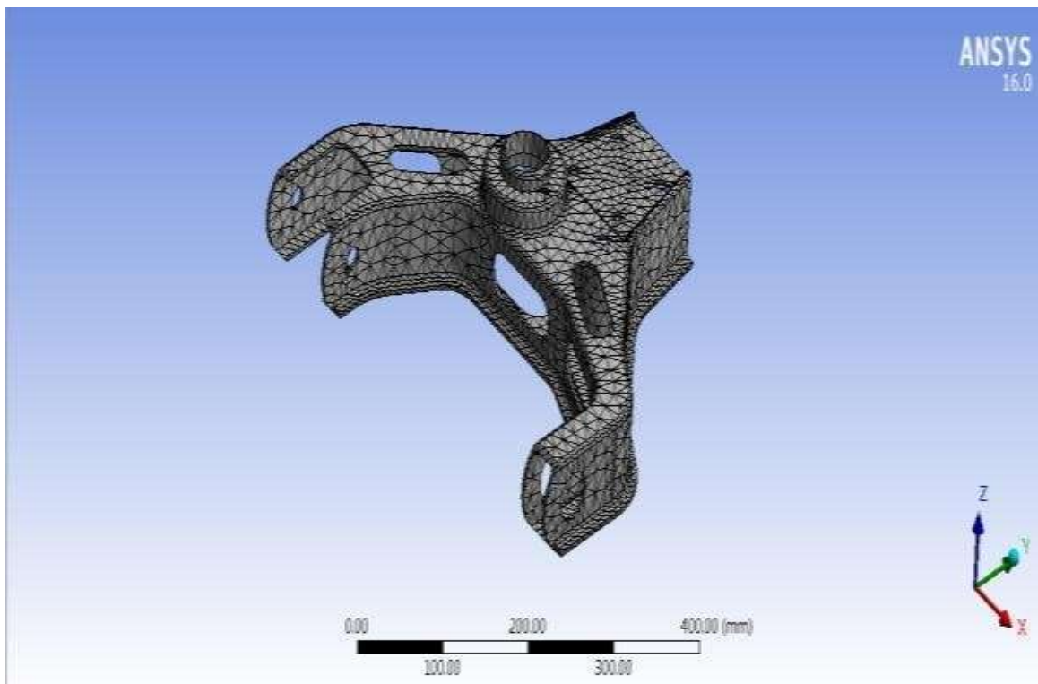
Fig 11: Meshing of UCM using tetrahedral element
