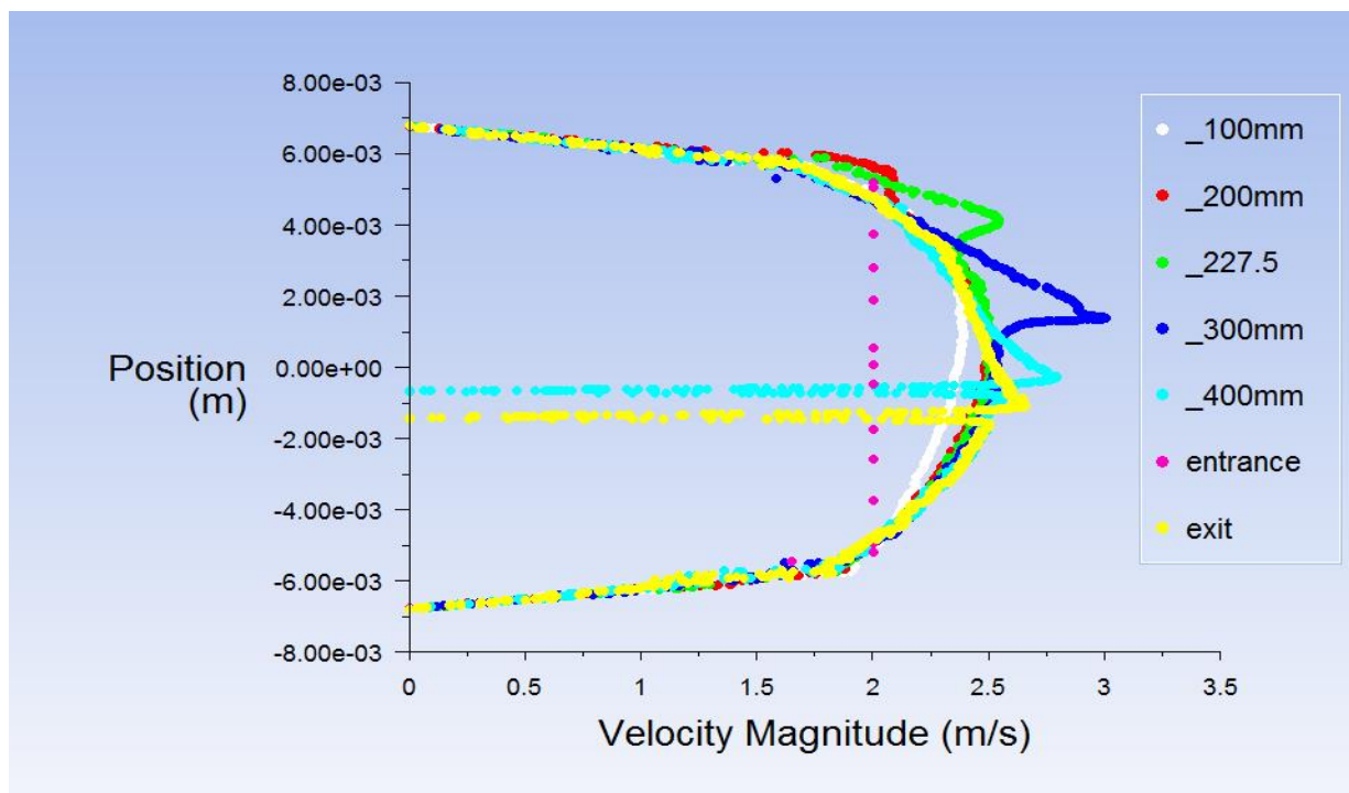
Fig-6: Velocity profile of 4Cored brick regenerator with inducer just after the developing length at different position
