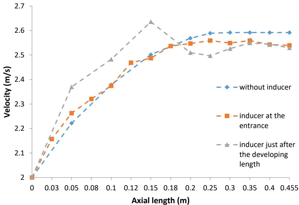
Chart-7: Axial velocity variation for different position of inducer and without inducer in 4Cored brick regenerator
