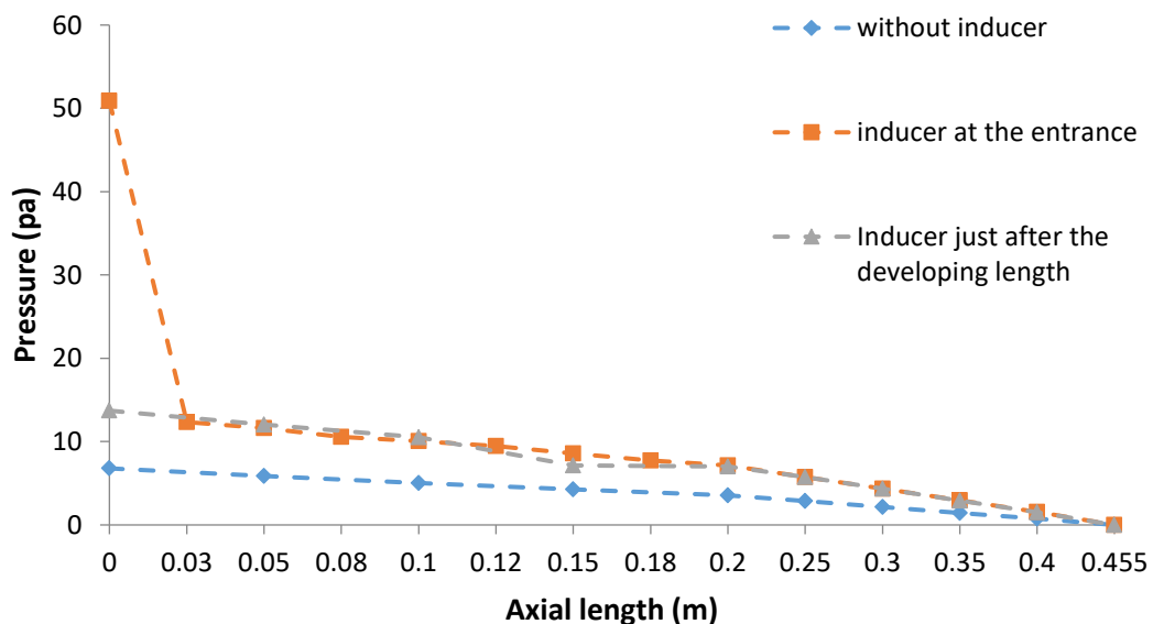
Chart- 8: Pressure variation along axial length for different position of inducer and without inducer in 4Cored brick regenerator
