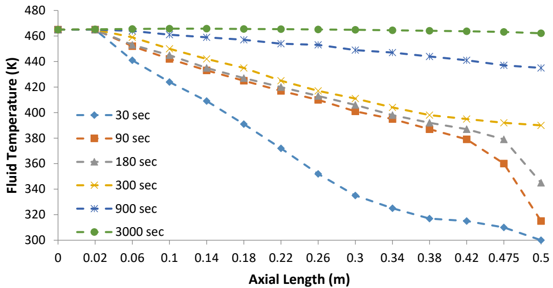
Chart-9: Average fluid temperature variation in 4Cored brick regenerator without inducer at different time
