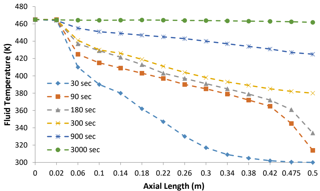
Chart-10: Average fluid temperature variation in 4Cored brick regenerator with inducer at the entrance at different time
