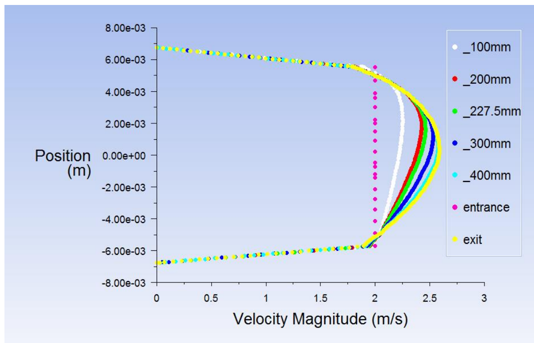
Fig-4: Velocity profile of 4Cored brick regenerator without inducer at different position
