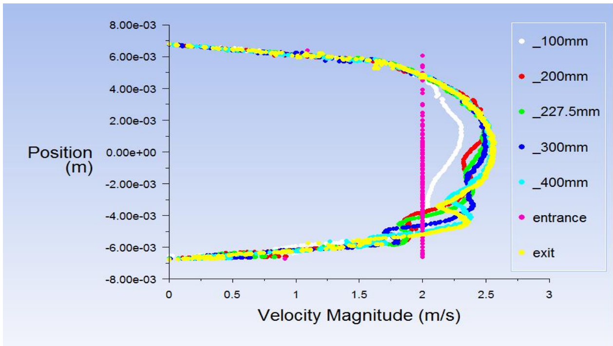
Fig-5: Velocity profile of 4Cored brick regenerator with inducer at the entrance at different position
