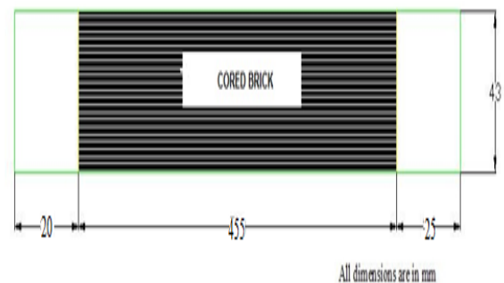
Fig-1: Sketch of Cored brick of CFD analysis
