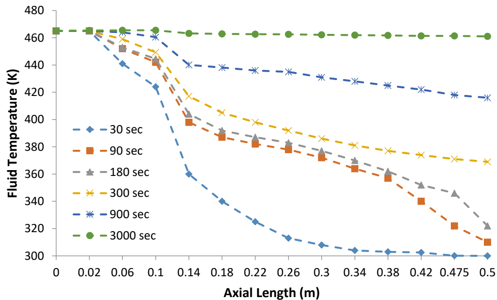
Chart-11: Average fluid temperature variation in 4Cored brick regenerator with inducer just after the developing length at different time
