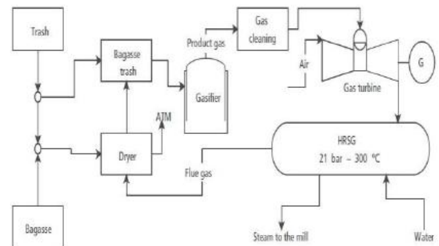
Fig 2 Simplified diagram of BIG plant integrated with the mill
