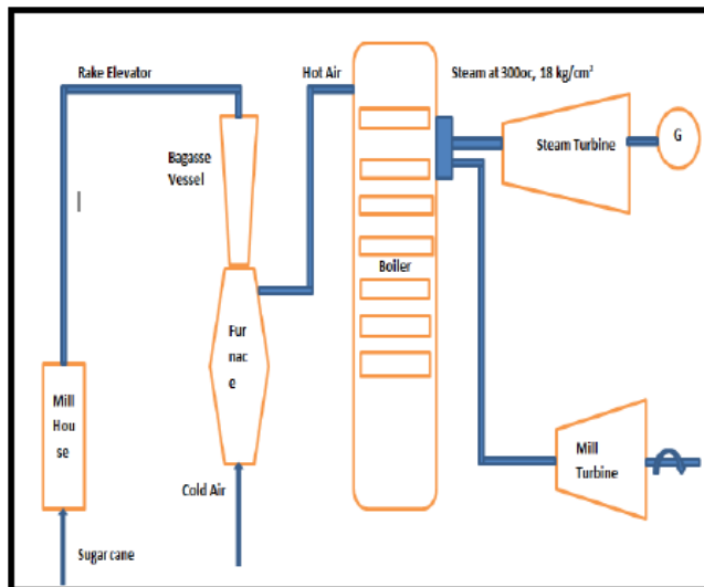
Fig 1 Schematic diagrams for a Condensing Extraction Steam Turbine (CEST) in Kisan Sahkari Chini Mills Ltd, Sultanpur
