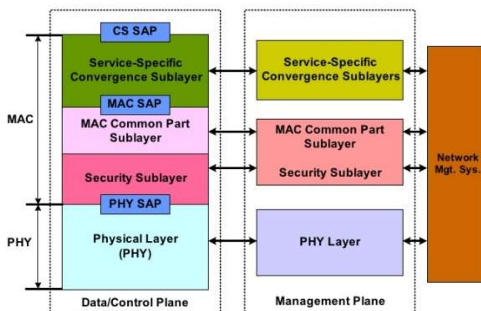
Fig. 1 - 802.16 Protocol and Standard
