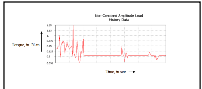
Load-time history
