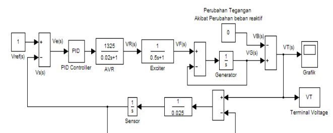
Fig-5: AVR simulation with proportional control on Normal Conditions (Load Changes = 0 due to changes Reactive Power = 0)
