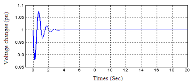
Fig-10: Results of simulation AVR with PID controller on normal condition with K_p = 0.0161354 , K_i = 0.04186340 and K_d = 0.00155477
