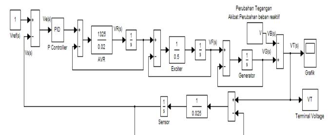
Fig-7: AVR simulation with P controller on the load condition.
