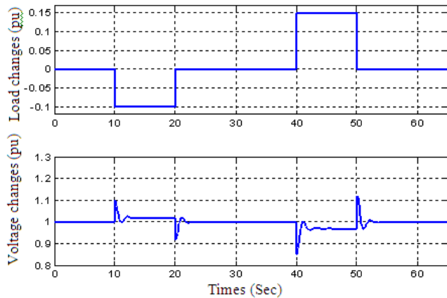
Fig-8: Simulation AVR with P controller when there disturbance.
