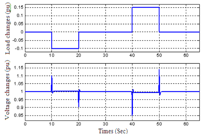
(b) Load decreased by 0.2 pu and load increase by 0.25 pu
