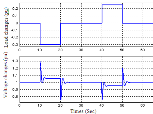
Fig-9: Results of simulation AVR with P controller when there disturbance.
