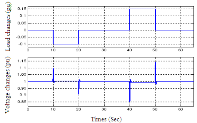
(a) Load decreased by 0.1 pu and load increase by 0.15 pu
