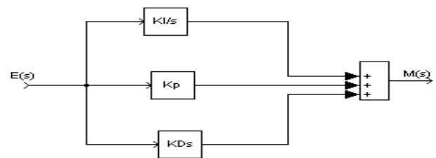
Fig-3: Block diagram of PID with Laplace
