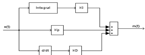
Fig-2: Block diagram of PID mathematically
