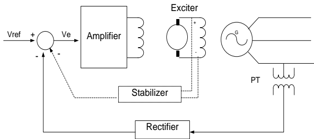
Fig-1: General Model of AVR [4]
