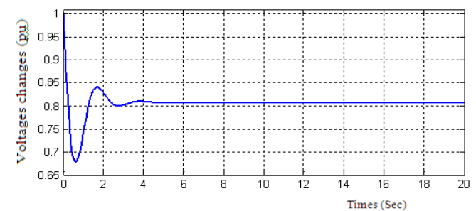
Fig-6: Relation output voltage versus time with K_p = 0.00318671
