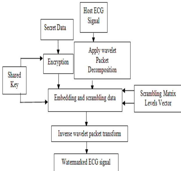
Fig -2: Block diagram of the sender steganography
