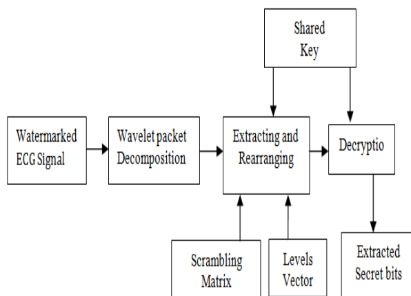
Fig - 7: Block diagram of the receiver steganography
