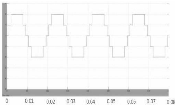
Fig 4.4 Generated output Waveform for the Middle Bridge Inverter.
