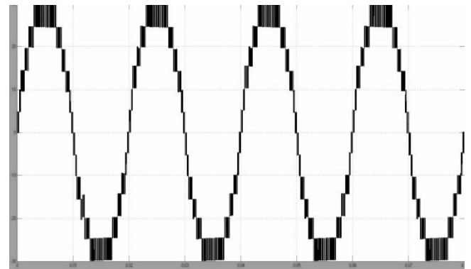
Fig 4.6 Total Output Voltage for the Proposed Cascaded H-Bridge Inverter
