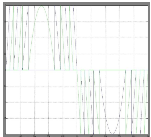
Fig 3.1 Reference Wave Signal Generation for the Upper Bridge Inverter
