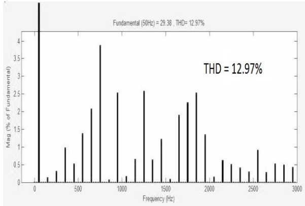
Fig 4.8 Line Voltage Harmonics with THD value
