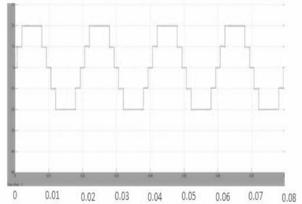
Fig 4.5 Generated output Waveform for the Lower Bridge Inverter.
