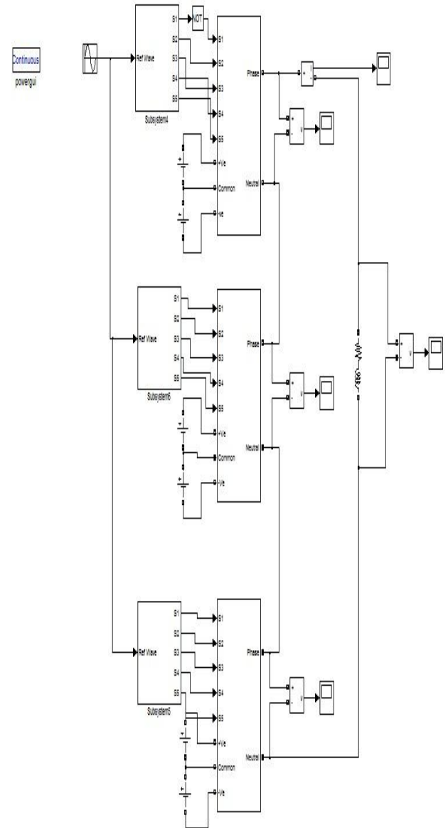
Fig 4.1 MATLAB/SIMULATION Diagram- Proposed Cascaded H-Bridge Multi-Level Inverter
