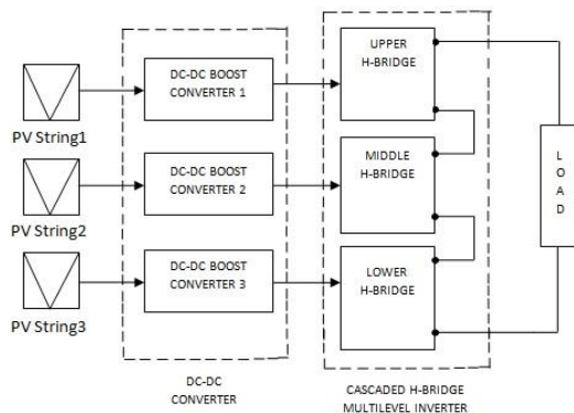
Fig. 1.1 Overall Block Diagram
