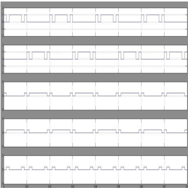
Fig 3.3 Generated Gate Pulses for Middle and Lower Bridge Switches
