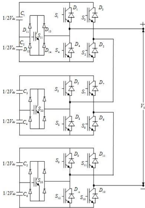
Fig. 2.1 Cell Configuration for the Proposed Inverter
