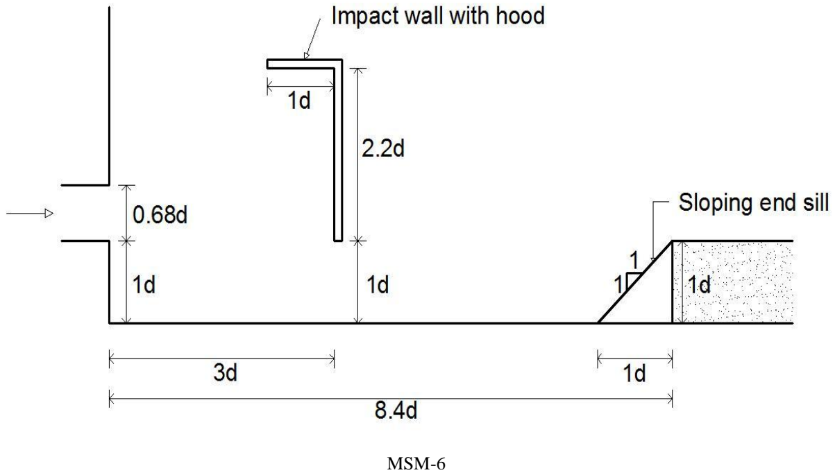
Fig 1 USBR VI Stilling basin model (Models MSM-6)
