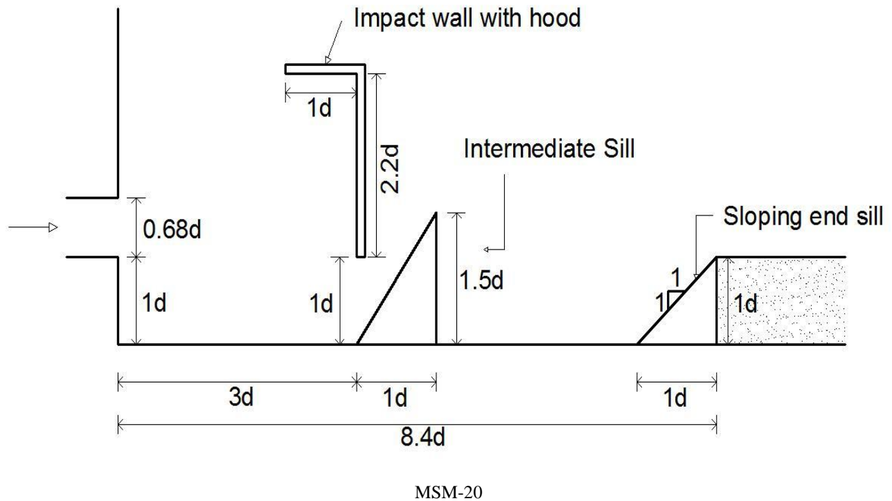
Fig 2 Model MSM-20 with USBR VI Impact Wall, Sloping End Sill and Intermediate Sill of height 1.5d with Vertical Face Downstream
