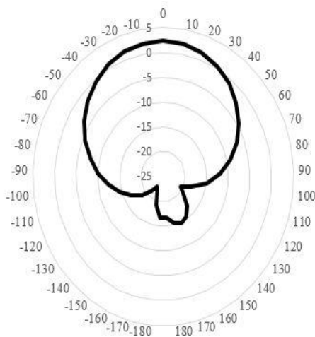
Fig-11 Radiation Pattern at 7.4 GHz
