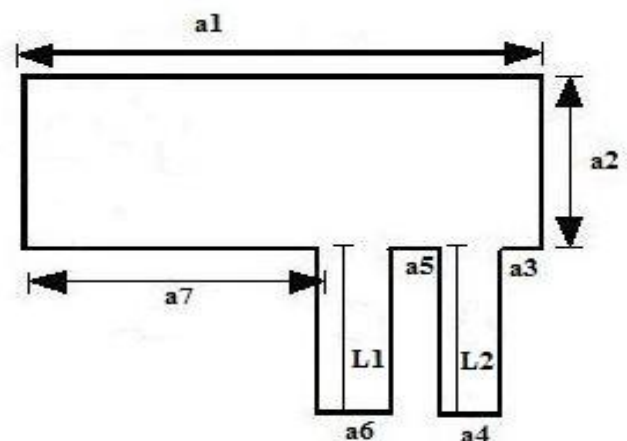
Fig -1 Geometry of the proposed rectangular patch antenna
