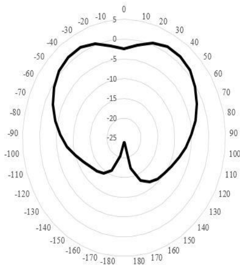
Fig-10 Radiation Pattern at 5.8 GHz
