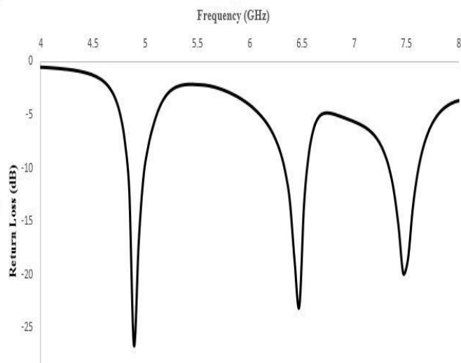
Fig-5 Return Loss of Patch 4
