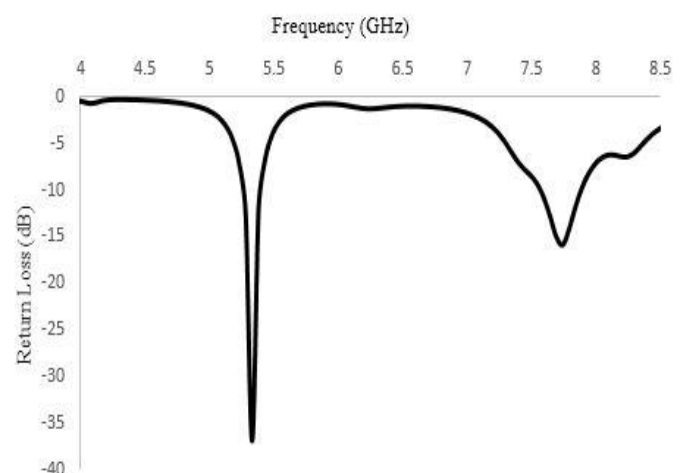
Fig-3 Return Loss of Patch 2
