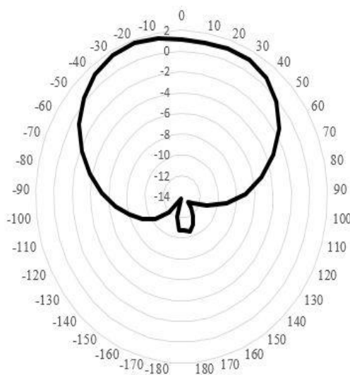
Fig-12 Radiation Pattern at 7.4 GHz
