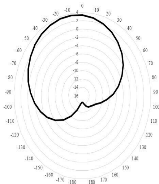
Fig-6 Radiation Pattern at 2.4 GHz
