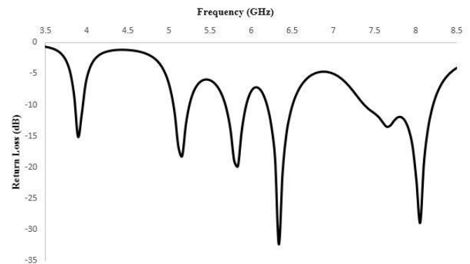
Fig-2 Return Loss of Patch 1
