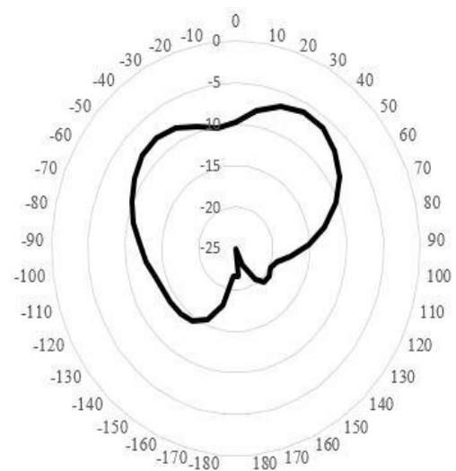
Fig-9 Radiation Pattern at 5.1 GHz
