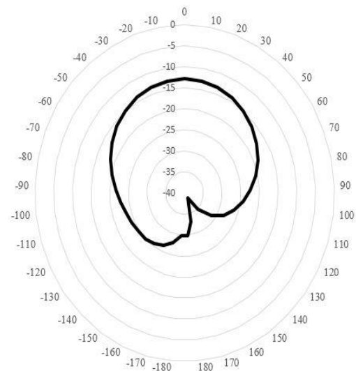
Fig-8 Radiation Pattern at 4.8 GHz
