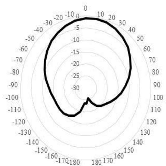
Fig-7 Radiation Pattern at 4.7 GHz
