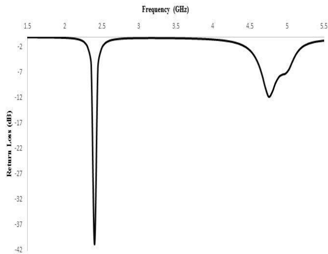
Fig-4 Return Loss of Patch 3
