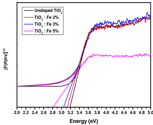
Fig -4: Tauc plot obtained from UV-Vis DRS spectrum of the as prepared undoped and Fe-doped nanoparticles.
