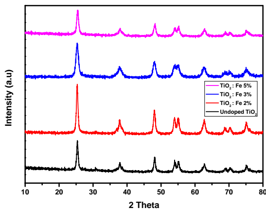
Fig -1: XRD patterns of as prepared undoped and Fe-doped Nano particles
