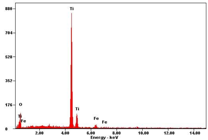
Fig -10: EDAX spectrum of the 2 wt% Fe doped Nano \text{TiO}_2 .
