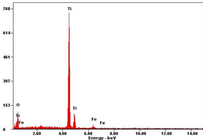
Fig -12: EDAX spectrum of the 5 wt% Fe-doped nano TiO 2 .
