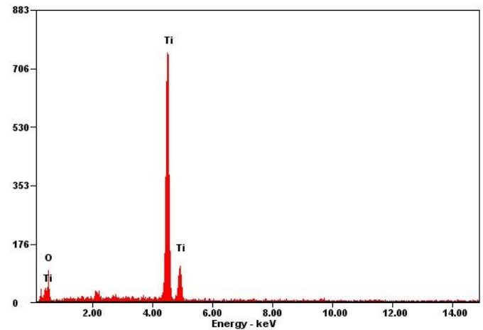
Fig -9: EDAX spectrum of the as prepared Nano \text{TiO}_2 .
