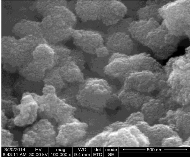
Fig -7: HR-SEM micrograph of the 3 wt% Fe-doped \text{TiO}_2 nanoparticles.
