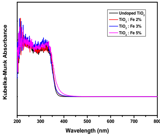
Fig -3: UV-Vis DRS spectrum of the as prepared undoped and Fe-doped nanoparticles.
