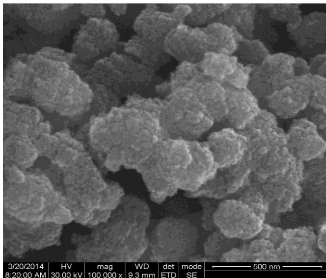
Fig -8: HR-SEM micrographs of the 5 wt% Fe-doped \text{TiO}_2 nanoparticles.
