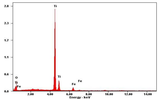
Fig -11: EDAX spectrum of the 3 wt% Fe-doped nano \text{TiO}_2 .
