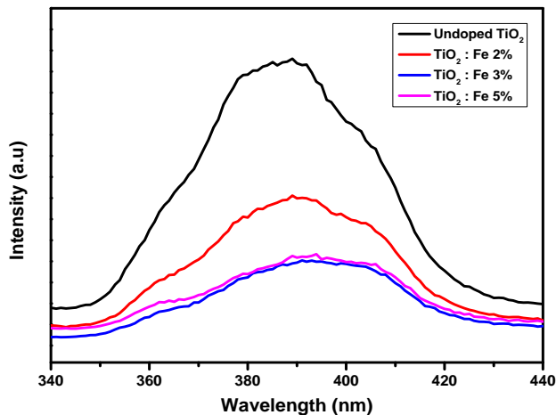
Fig -13: The Photoluminescence spectrum of as prepared undoped and Fe-doped nano TiO 2 .
