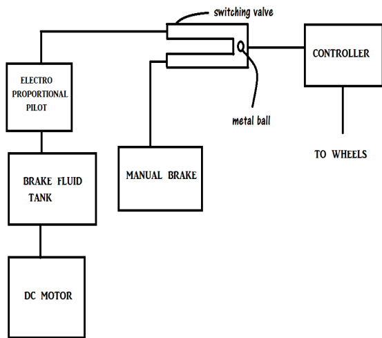
Fig.5 Diagram of Electro-Hydraulic Braking System
