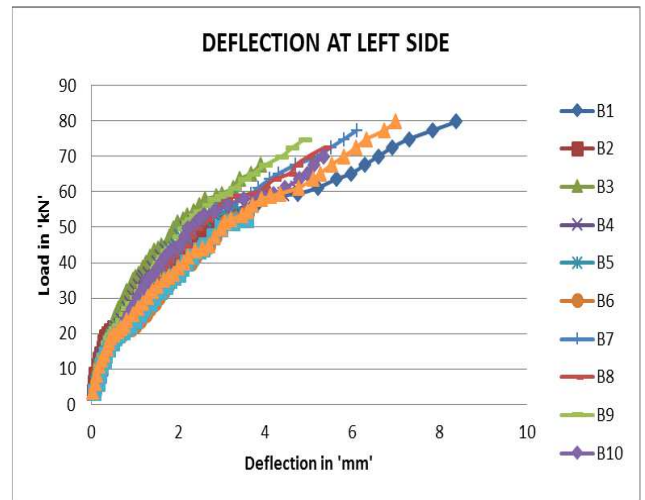
Fig. 5: Load-deflection relationship for all beams at left side
