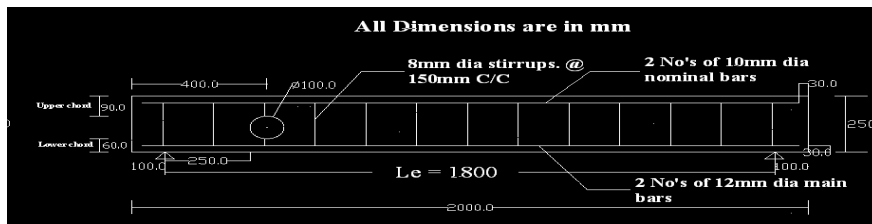
Fig. 1: Dimension of beam with circular opening in shear zone
