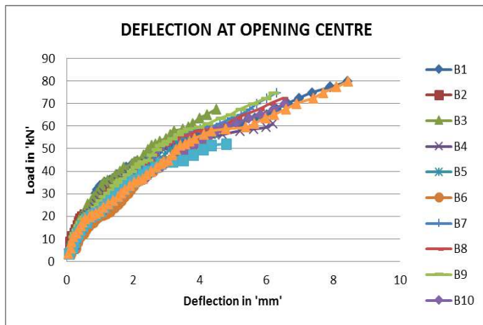
Fig. 4: Load-deflection relationship for all beams at the opening centre
