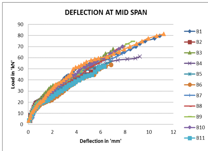
Fig. 3: Load-deflection relationship for all beams at mid span
