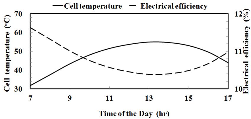
Fig.3: Hourly variations of cell temperature and electrical efficiency at \dot{m} = 0.005 \text{ kg/s}
