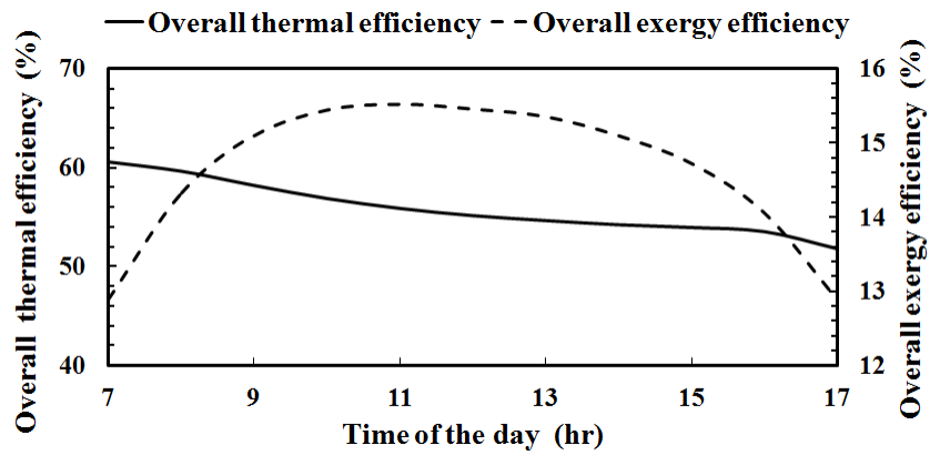
Fig.4: Hourly variations of overall thermal and overall exergy efficiency at \dot{m} = 0.005 \text{ kg/s}
