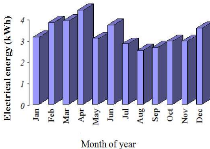
Fig.5: Month wise electrical energy kWh
