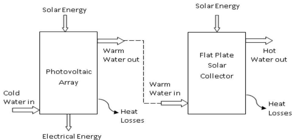
Fig.1 Schematic diagram of PVT and FPC connected in series
