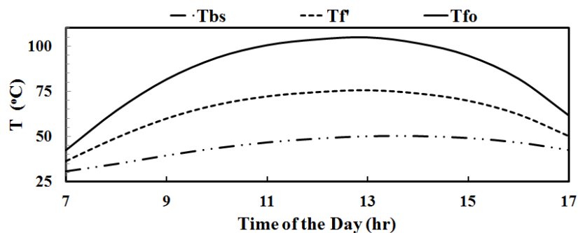
Fig.2 Hourly variations of water outlet temperature from FPC and PVT and back surface of the solar cell at \dot{m} = 0.005 \text{ kg / s}
