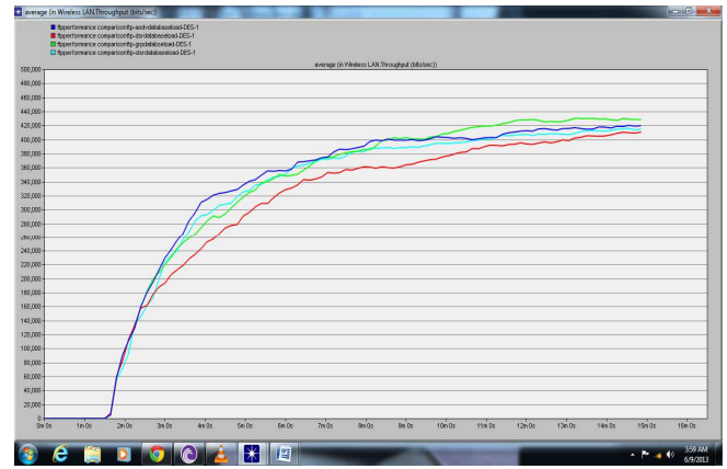
Figure 19: Comparison of DSR, AODV, GRP and OLSR Protocol for throughput in Database Load
