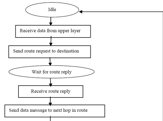
Figure 6: Flow Chart of sending activity diagram
