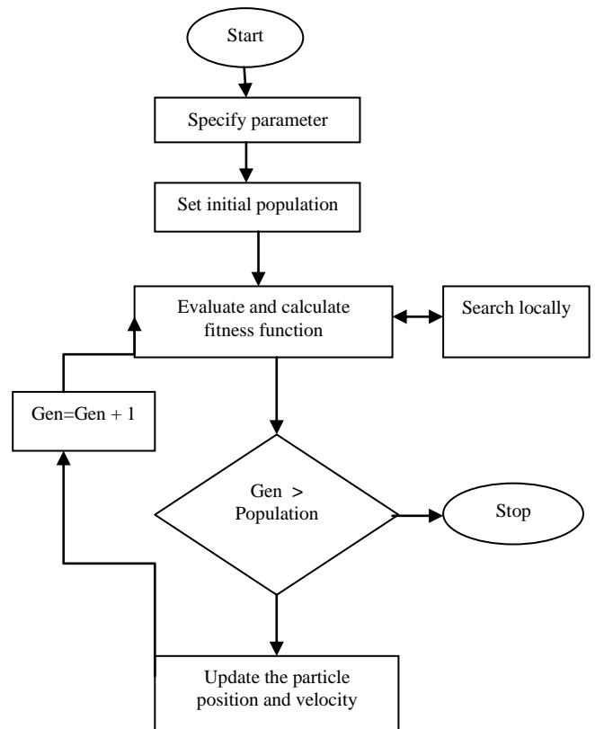
Figure2 Particle Swarm Optimization
