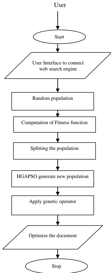
Figure5 Data flow diagram of HGAPSO
