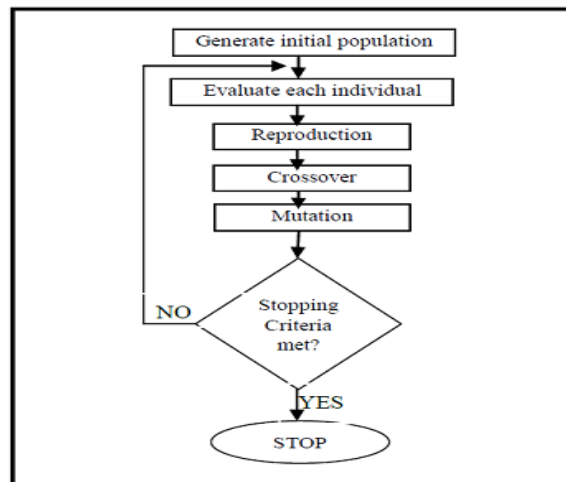
Figure 4. Flowchart of typical Genetic algorithm
