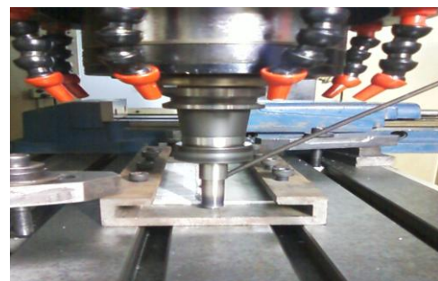
Figure 1. CNC milling machine with tool and fixture
