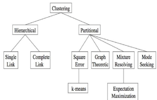
Fig 4: Clustering methods classifications for Moses Charikar [10]
